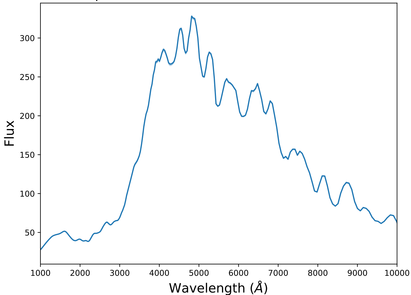
Spectrum 7 for transient CCSN at z=0.26
